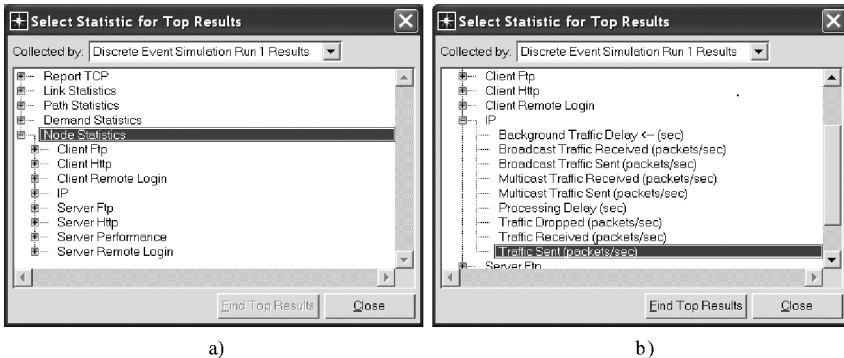
图 4.16 Select Statistics for Top Results 窗口
