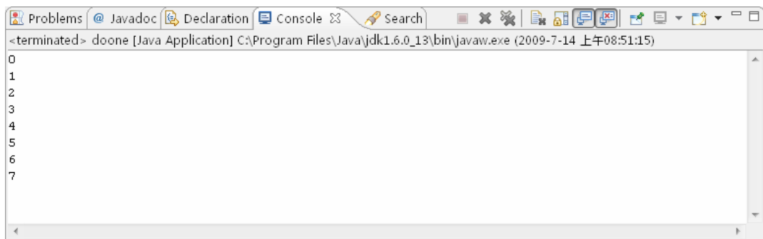
图 6-13 do...while 语句
